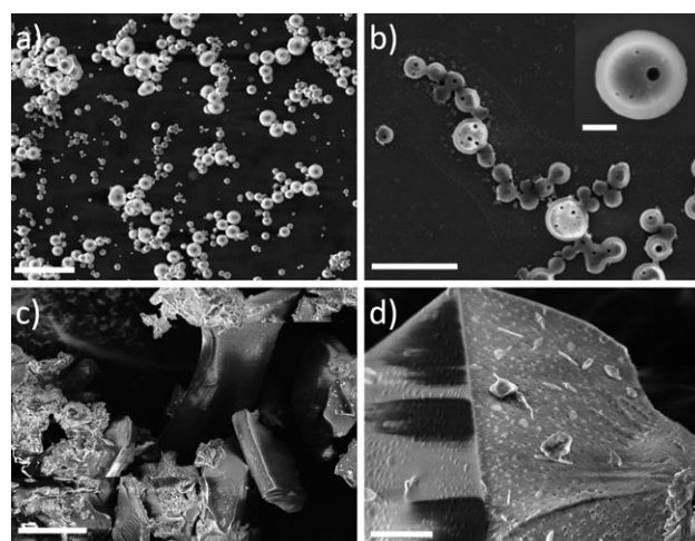
Figure 4. a,b) SEM images of hollow polymer nanosized superstructures prepared by drop-casting a dilute solution of 5\cdot n\text{PF}_6 , followed by removal of solvent under vacuum. SEM image (b, inset) of a single hollow polymer superstructure with clearly visible pores in the shell. c,d) SEM images of larger assembled superstructures prepared by slow solvent evaporation of 5\cdot n\text{PF}_6 on glass. The scale bars are a) 4 \mu\text{m} , b) 2 \mu\text{m} and 200 nm (inset), c) 20 \mu\text{m} , and d) 2 \mu\text{m} .
