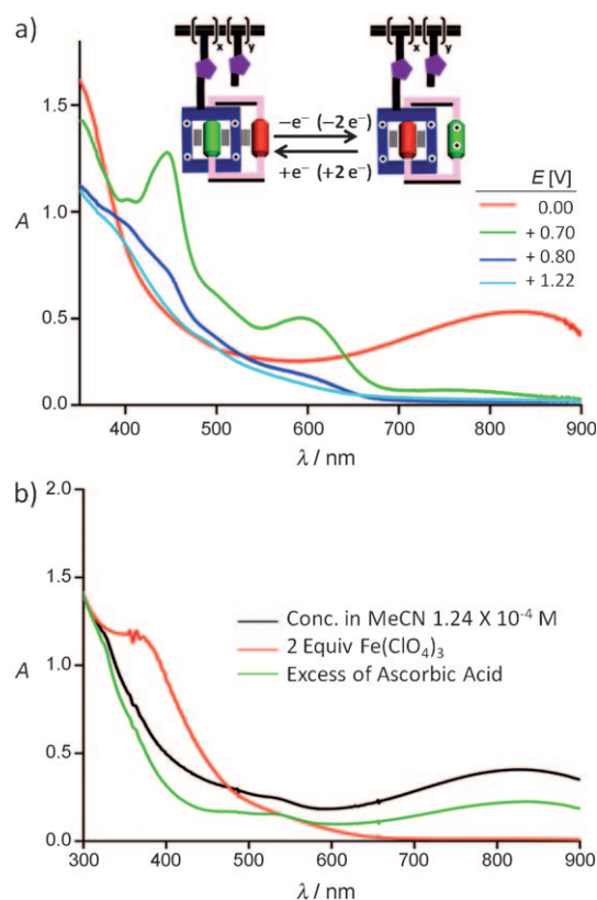
Figure 2. a) UV/Vis spectroelectrochemistry of the bistable poly[2]catenane 5-nPF 6 ( 5 \times 10^{-4} \text{ M} , MeCN, 0.1 \text{ M TBAPF}_6 , 298 K) recorded over a range of potentials illustrating the reversible two-electron electrochemically induced switching behavior of the bistable [2]catenane polymer side chains (inset). b) UV/Vis absorption spectra of the bistable poly[2]catenane 5-nPF 6 ( 1.24 \times 10^{-4} \text{ M} , MeCN, 298 K) illustrating the reversible chemically induced switching after the addition of 2 equivalents of the chemical oxidant \text{Fe}(\text{ClO}_4)_3 and reduction with an excess of ascorbic acid.
