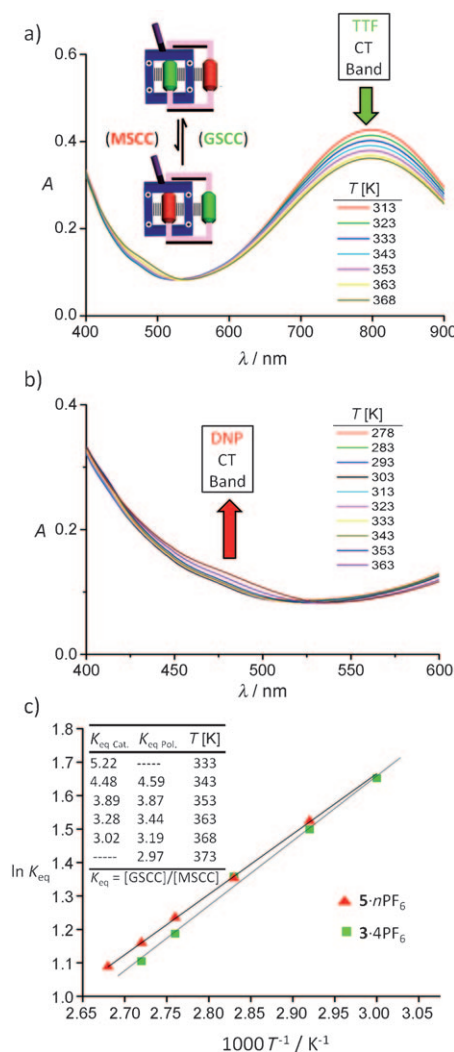
Figure 1. a) Variable temperature UV/Vis spectra of the alkyne-functionalized [2]catenane 3 ·4PF 6 and b) the side-chain poly[2]catenane 5 · n PF 6 ( 2 \times 10^{-4} \text{ M} , DMF) illustrating the temperature-dependent equilibrium (inset) between the GSCC (TTF-CBPQT 4+ charge-transfer band at 800 nm) and MSCC (DNP-CBPQT 4+ charge-transfer band at 480 nm). c) Linear Van't Hoff plots for 3 ·4PF 6 ( R^2=0.996 ) and 5 · n PF 6 ( R^2=0.996 ) for the thermally induced GSCC→MSCC equilibrium (inset); the \Delta G^\circ_{298K} , \Delta H^\circ , and \Delta S^\circ values for the process were obtained as described in the footnotes to Table 1.
