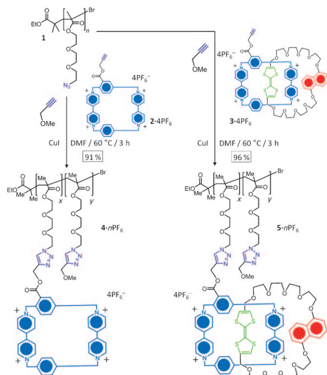
Scheme 1. Click functionalization of polymer 1 ( n=160 ) with the alkyne-functionalized tetracationic cyclophane 2 ·4PF 6 and the alkyne-functionalized bistable [2]catenane 3 ·4PF 6 for the formation of 4 · n PF 6 ( x=27 , y=133 ) and 5 · n PF 6 ( x=42 , y=118 ).
